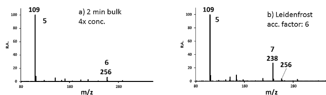
Figure 2. The bulk-phase reaction of 4 and 5 showed mainly reagent 5 and a small amount of intermediate 6 after 2 min (a) whereas the parallel Leidenfrost experiment led to significant product ( 7 ) formation (b).
